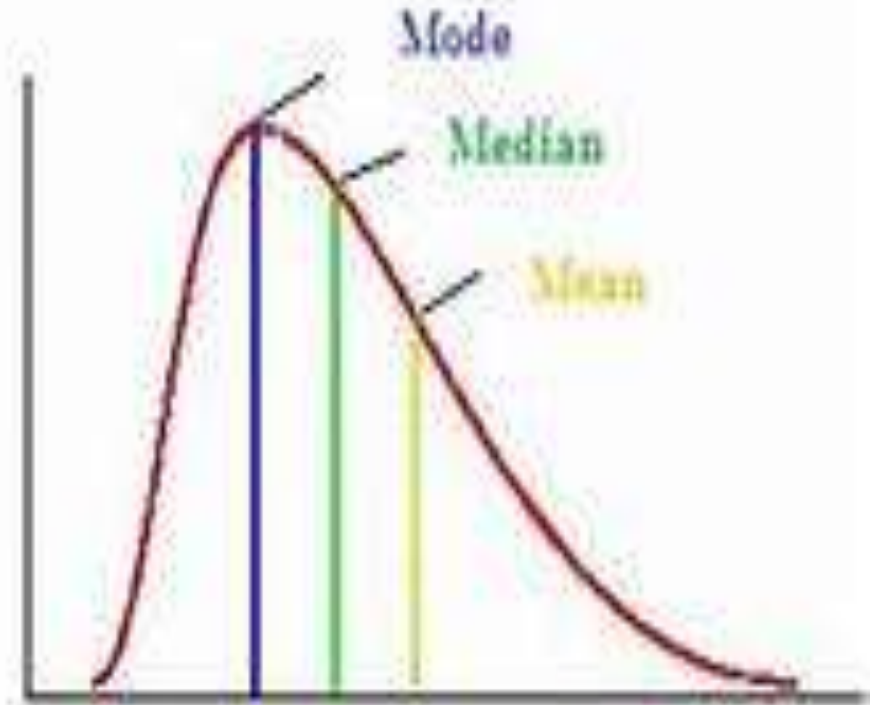
Right-Skewed (Positive Skewness)
