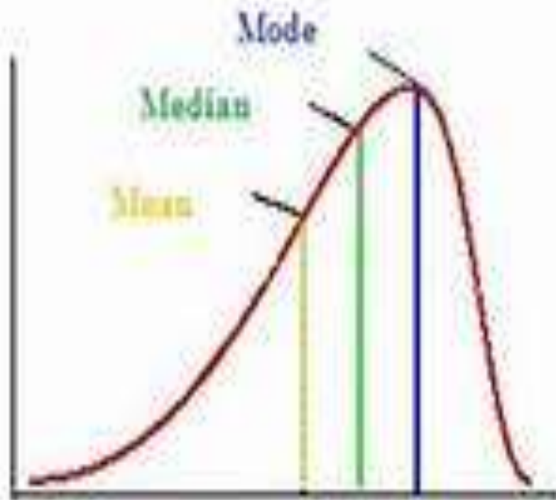
Left-Skewed (Negative Skewness)
